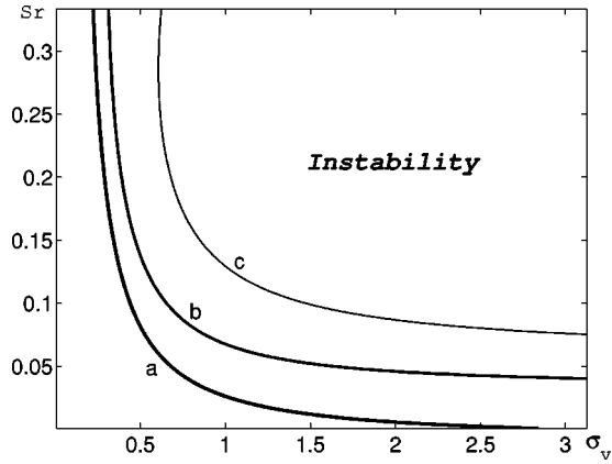
FIG. 2. The range of parameters ( Sr, \sigma_v ) for \tilde{Sc}=10^3 (curve c), \tilde{Sc}=10^5 (curve b), and \tilde{Sc}\rightarrow\infty (curve a). The line Sr=0 corresponds to the \delta -correlated in time random compressible velocity field.
